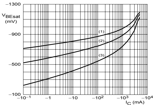
I_C/I_B = 10. (1) T_{amb} = -55\text{ }^{\circ}C. (2) T_{amb} = 25\text{ }^{\circ}C. (3) T_{amb} = 150\text{ }^{\circ}C.
