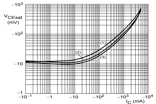
I_C/I_B = 20. (1) T_{amb} = 150\text{ }^{\circ}C. (2) T_{amb} = 25\text{ }^{\circ}C. (3) T_{amb} = -55\text{ }^{\circ}C.
