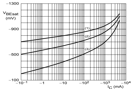
I_C/I_B = 20. (1) T_{amb} = -55\text{ }^{\circ}C. (2) T_{amb} = 25\text{ }^{\circ}C. (3) T_{amb} = 150\text{ }^{\circ}C.
