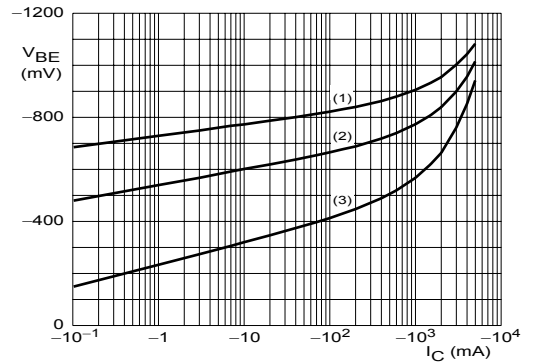
V_{CE} = -2 V. (1) T_{amb} = -55\text{ }^{\circ}C. (2) T_{amb} = 25\text{ }^{\circ}C. (3) T_{amb} = 150\text{ }^{\circ}C.
