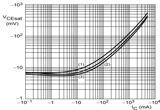
I_C/I_B = 10. (1) T_{amb} = 150\text{ }^{\circ}C. (2) T_{amb} = 25\text{ }^{\circ}C. (3) T_{amb} = -55\text{ }^{\circ}C.
