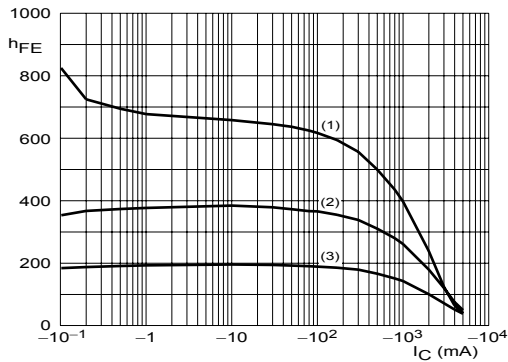
V_{CE} = -2 V. (1) T_{amb} = 150\text{ }^{\circ}C. (2) T_{amb} = 25\text{ }^{\circ}C. (3) T_{amb} = -55\text{ }^{\circ}C.
