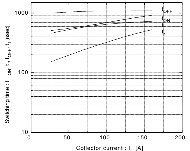
Switching time vs. Collector current V_{CC}=600\text{V}, R_G=9.1\Omega, V_{GE}=\pm 15\text{V}, T_j=125^\circ\text{C}
