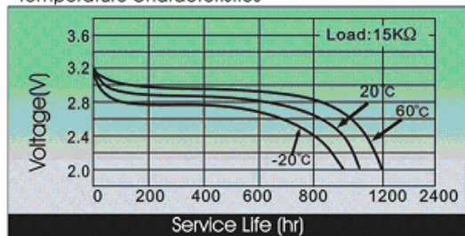
Temperature Characteristics
