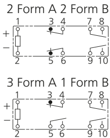
Schematic ( BOTTOM VIEW ) Standard
