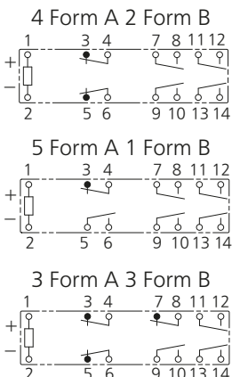
Schematic ( BOTTOM VIEW ) Standard
