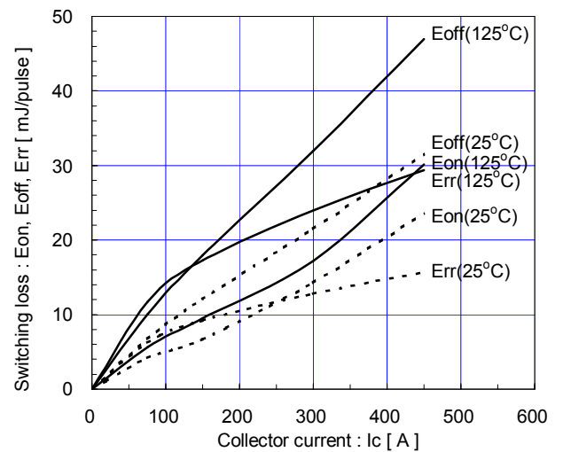
Switching loss vs. Collector current (typ.) V_{CC}=600V, V_{GE}=\pm 15V, R_G=2.0\Omega
