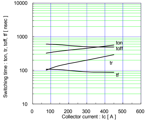
Switching time vs. Collector current (typ.) V_{CC}=600V, V_{GE}=\pm 15V, R_G=2.0\Omega, T_J=125^\circ C
