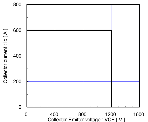
Reverse bias safe operating area (max.) +V_{GE}=15V, -V_{GE} \le 15V, R_G \ge 2.0\Omega, T_J \le 125^\circ C
