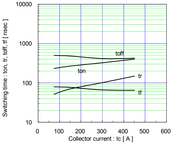
Switching time vs. Collector current (typ.) V_{CC}=600V, V_{GE}=\pm 15V, R_G=2.0\Omega, T_J=25^\circ C
