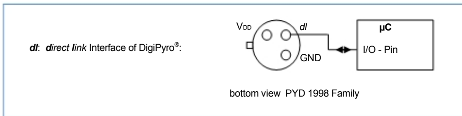
Figure 2 DigiPyro ® connections
