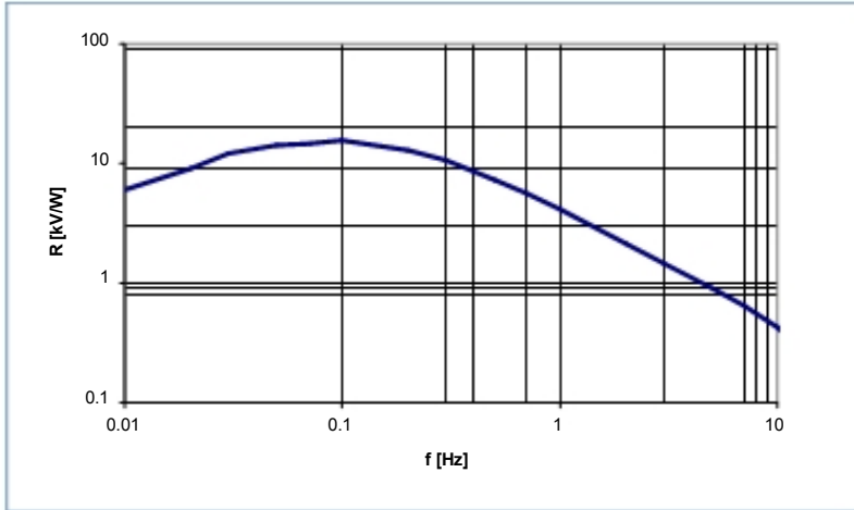
Figure 5 Frequency response
