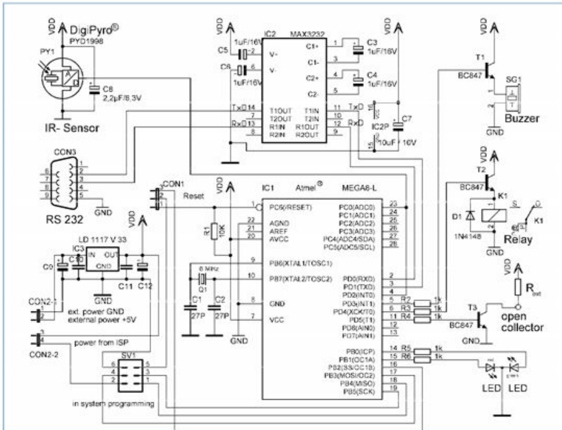
Fig.6 Typical application circuit
