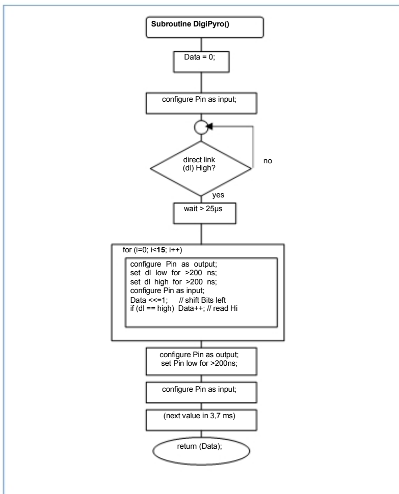
Figure 4 DigiPyro ® read-out flow chart
