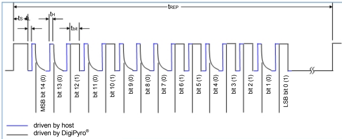
Figure 3 ADC and data transmission diagram (transmitted value: 146 D Hex = 5299 Dez )
