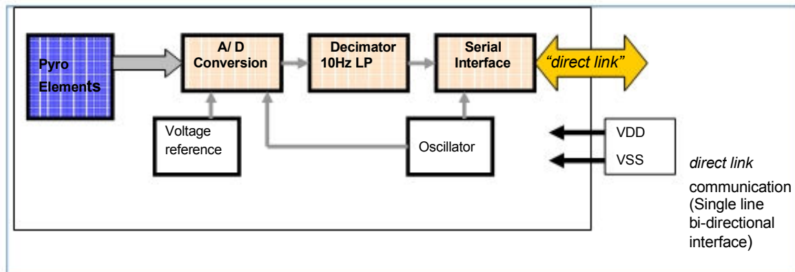
Figure 1 Block diagram of DigiPyro®
