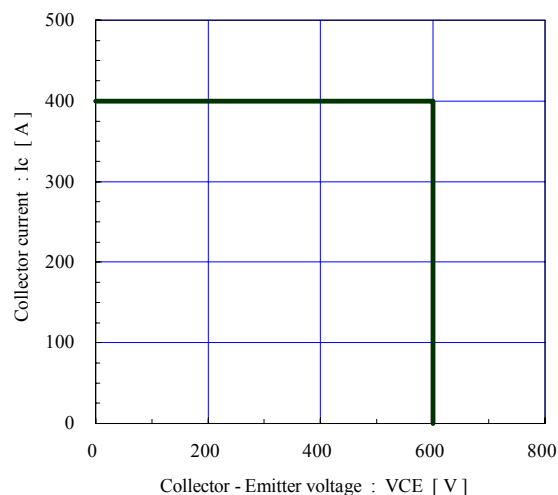
Reverse bias safe operating area (max.) +V_{GE}=15V, -V_{GE} \leq 15V, R_g \geq 16\Omega, T_j \leq 125^\circ C
