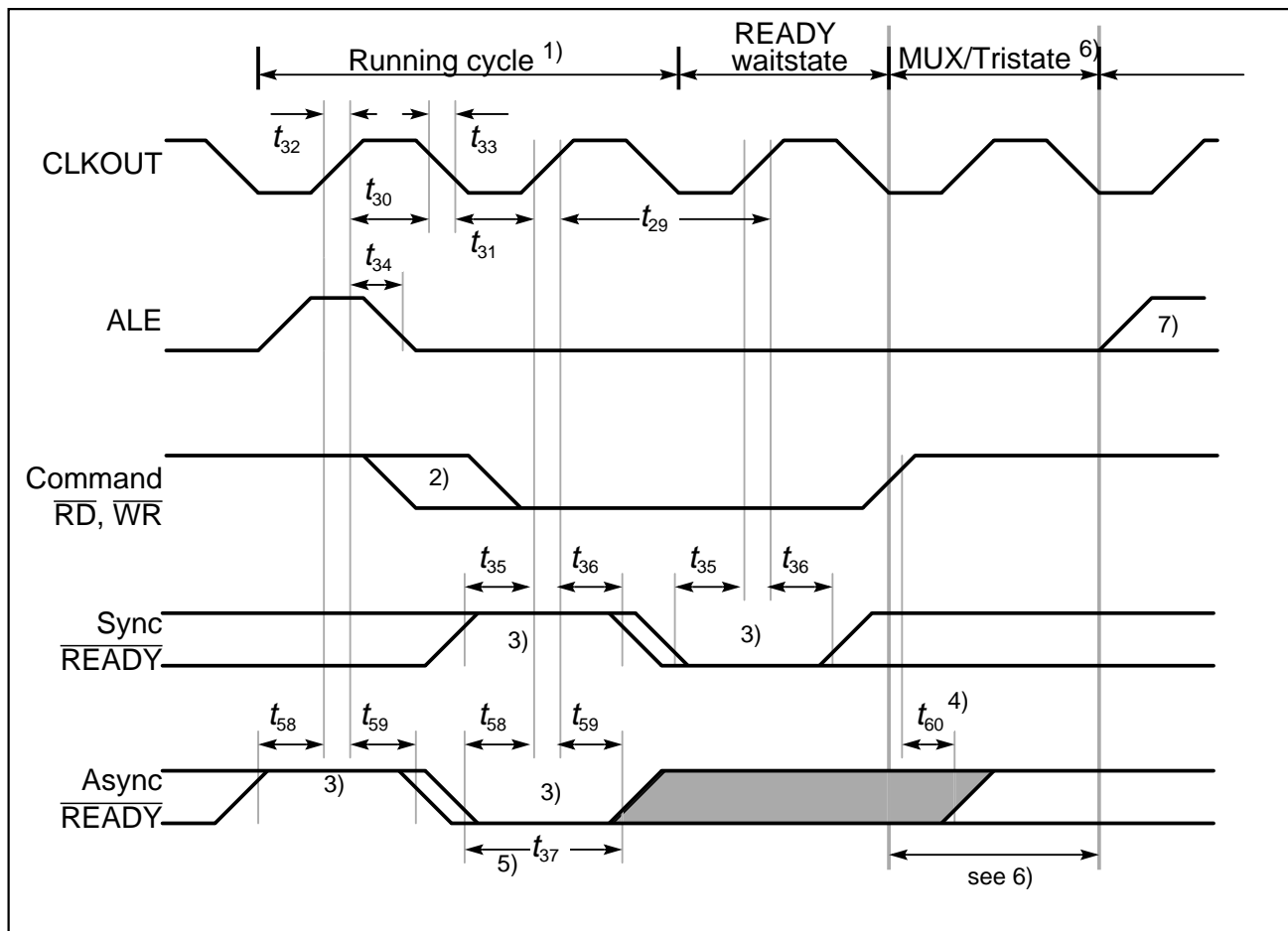
Figure 25 CLKOUT and READY
