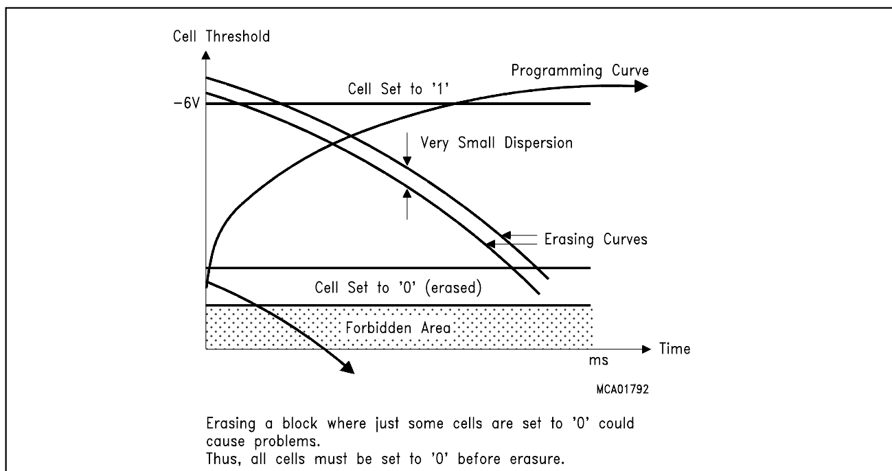
Figure 11 Flash Erasure
