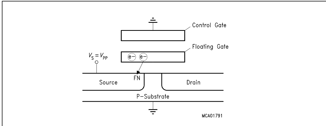
Figure 10 Flash Memory Cell Erase Mechanism
